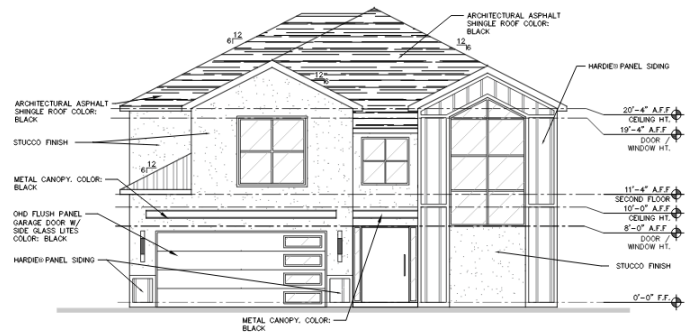
FRONT ELEVATION - CONTEMPORARY 2 STORY
