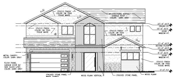
FRONT ELEVATION - CONTEMPORARY 2 STORY
