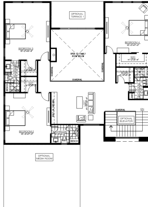
FLOOR PLAN - SECOND LEVEL
