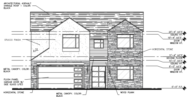
FRONT ELEVATION - CONTEMPORARY 2 STORY
