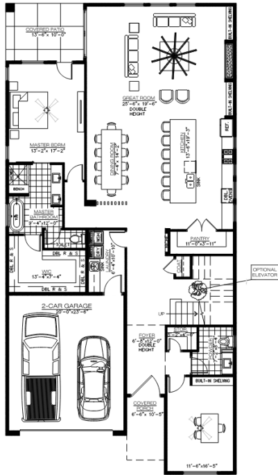
FLOOR PLAN - FIRST LEVEL
